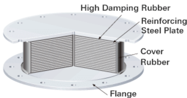
Figure 3. 3 High Damping Rubber Bearing
