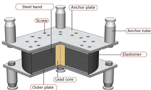
Figure 3.2: Elastomeric isolation system
