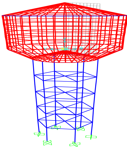
Figure 1: Fixed Base Structure in SAP2000
