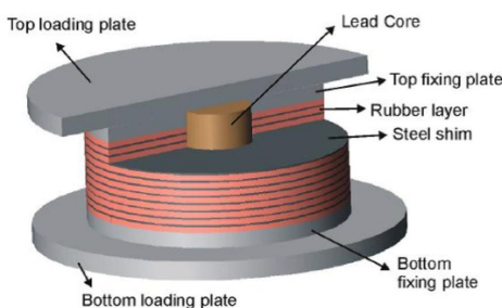
Figure 3.2: Lead Rubber Bearing
