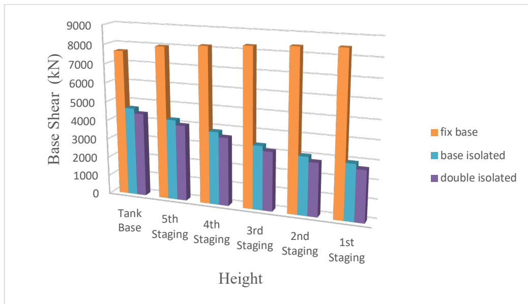
Figure 2: Comparison graph between fix base structure, base isolated structure and double isolated structure for base shear
