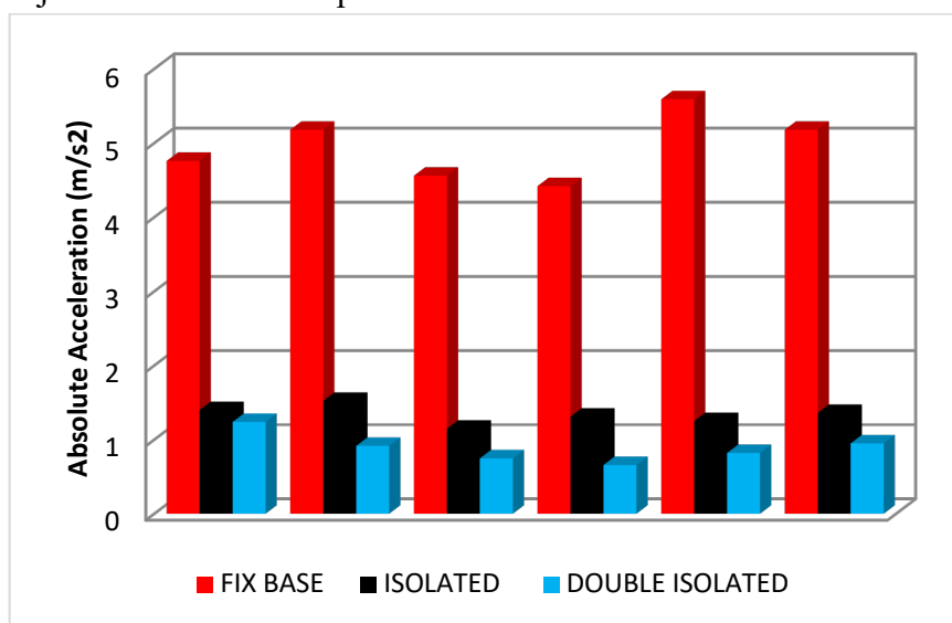
Figure 3: Comparison graph between fix base structure, base isolated structure and double isolated structure for absolute acceleration
