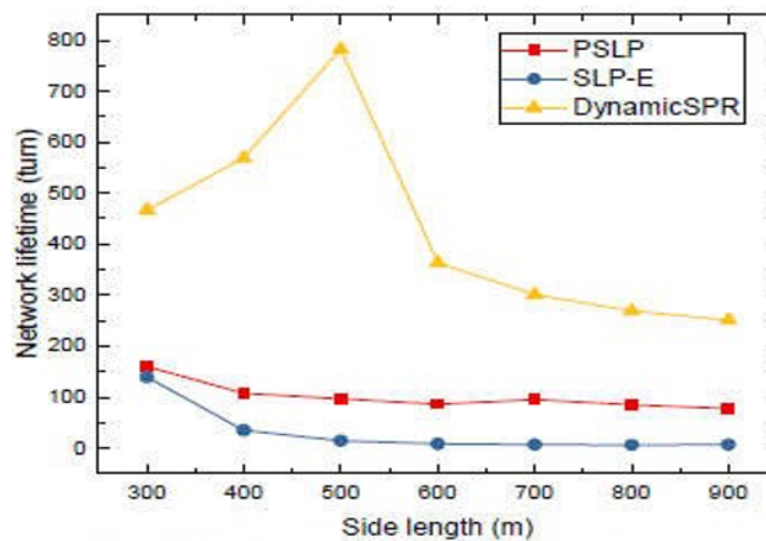
Figure 4: Network Lifetime of Three Schemes with Various Routes
