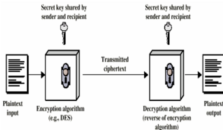
Figure 1: A Simplified Model of Conventional Encryption
