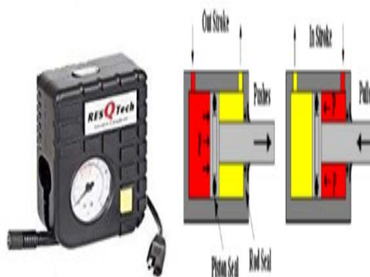
Figure 2: Inflator used pneumatic air cylinders
